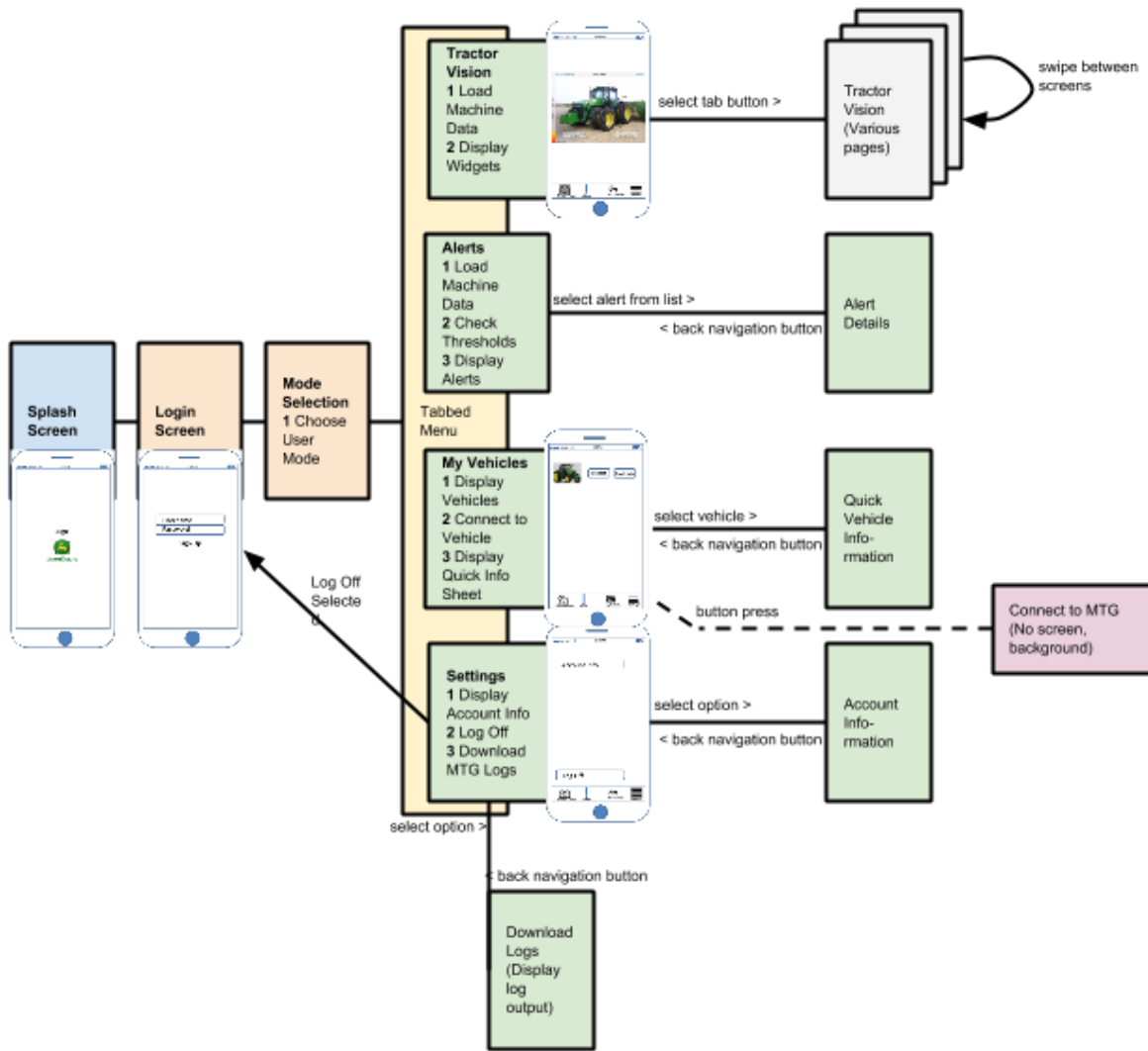
Figure 1: Tentative Screenflow for Application Transitions
